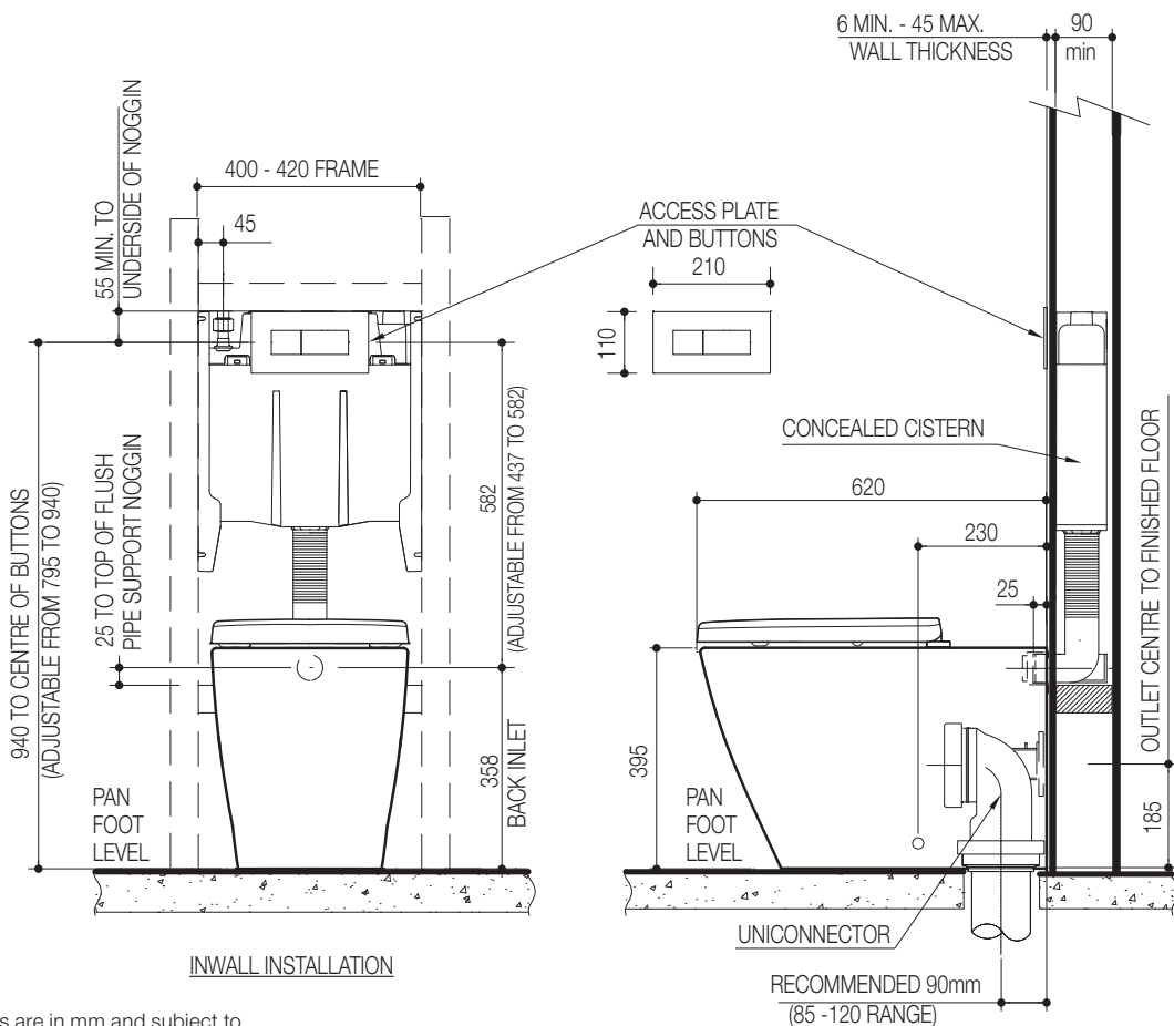
Drawing Scale 1:15
